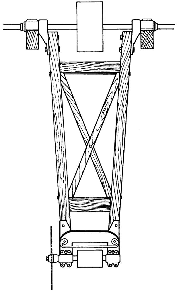
Figure 8-24. Single cutoff trim saw.
